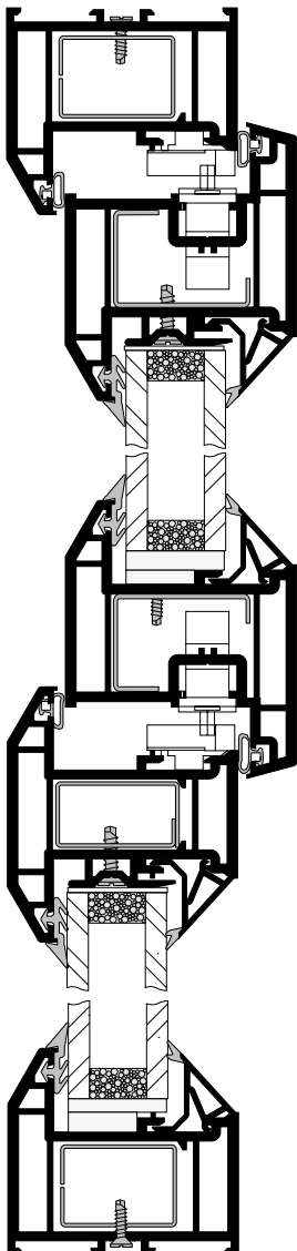
General assembly, internally glazed
