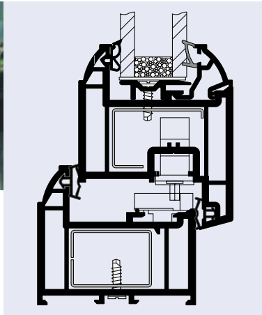
Intermediate outerframe with tilt and turn sash
