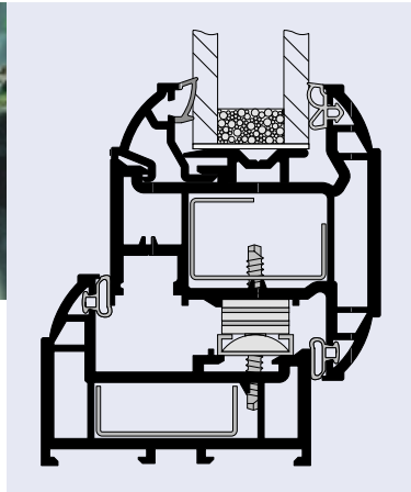
Featured slim outerframe with internally beaded sash
